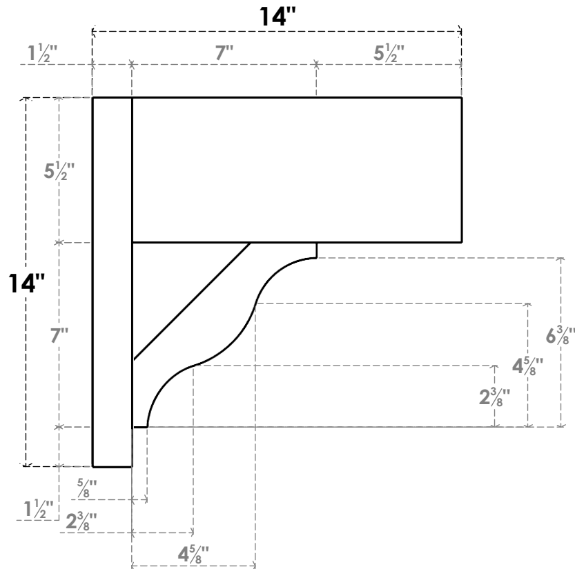
SIDE PROFILE
